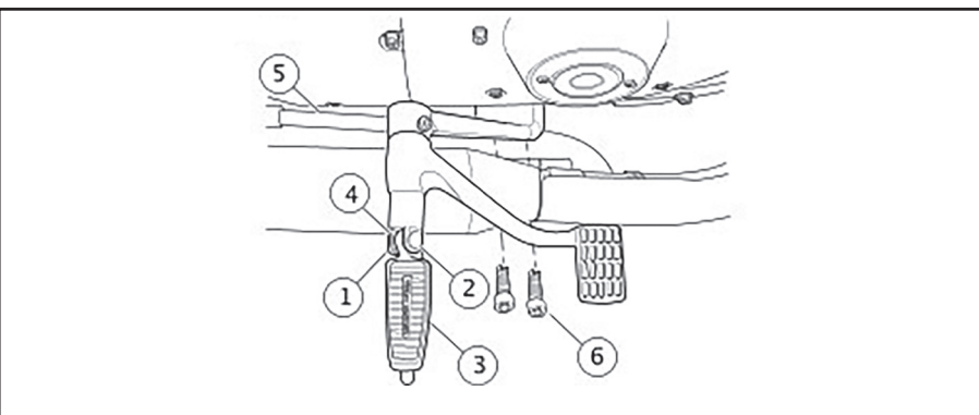
Figure 3. Remove Footrest Support and Brake Pedal
