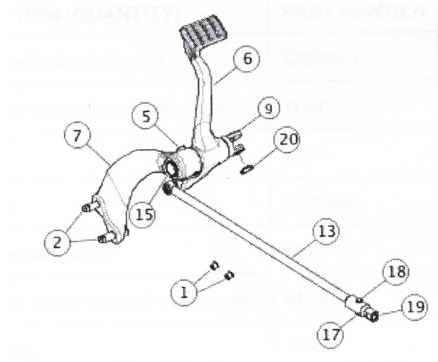
Figure 6. Service Parts: Forward Control Right (Brake) Side
