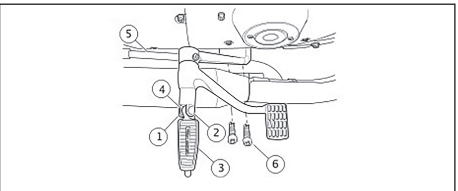
Figure 3. Remove Footrest Support and Brake Pedal
