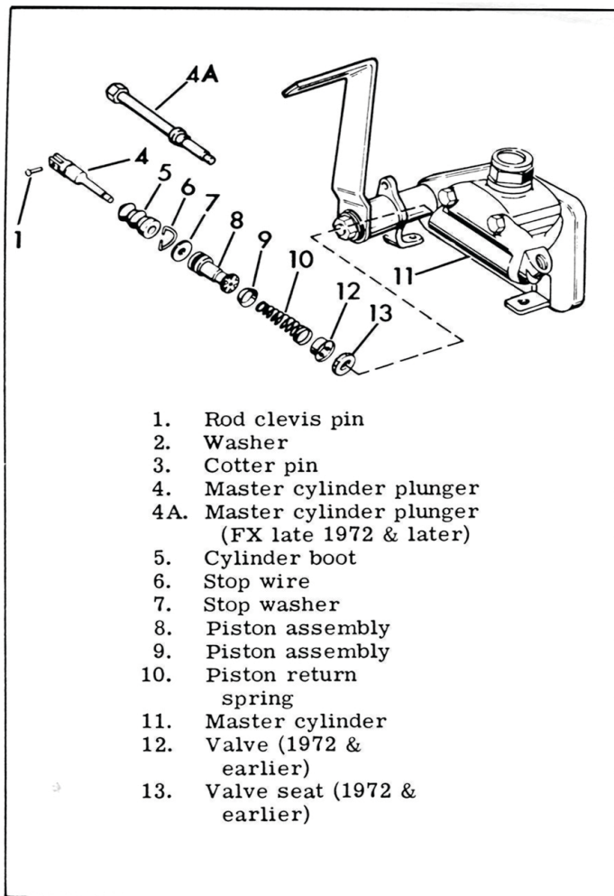
Figure 2-44A. Rear Brake Master Cylinder - Exploded View
