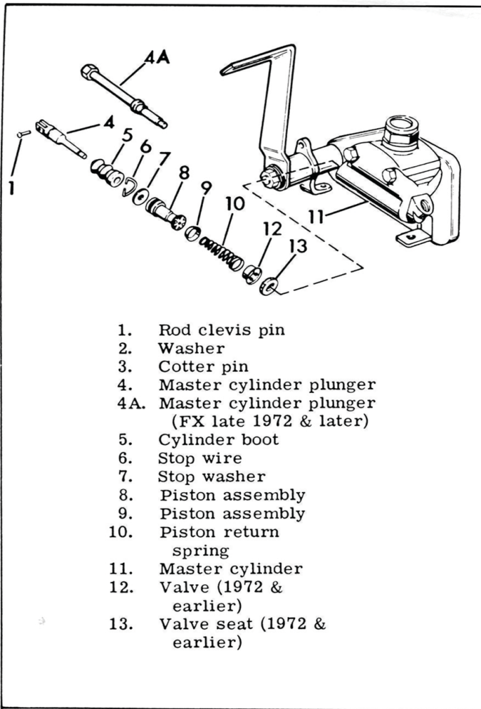
Figure 2-44A. Rear Brake Master Cylinder - Exploded View
