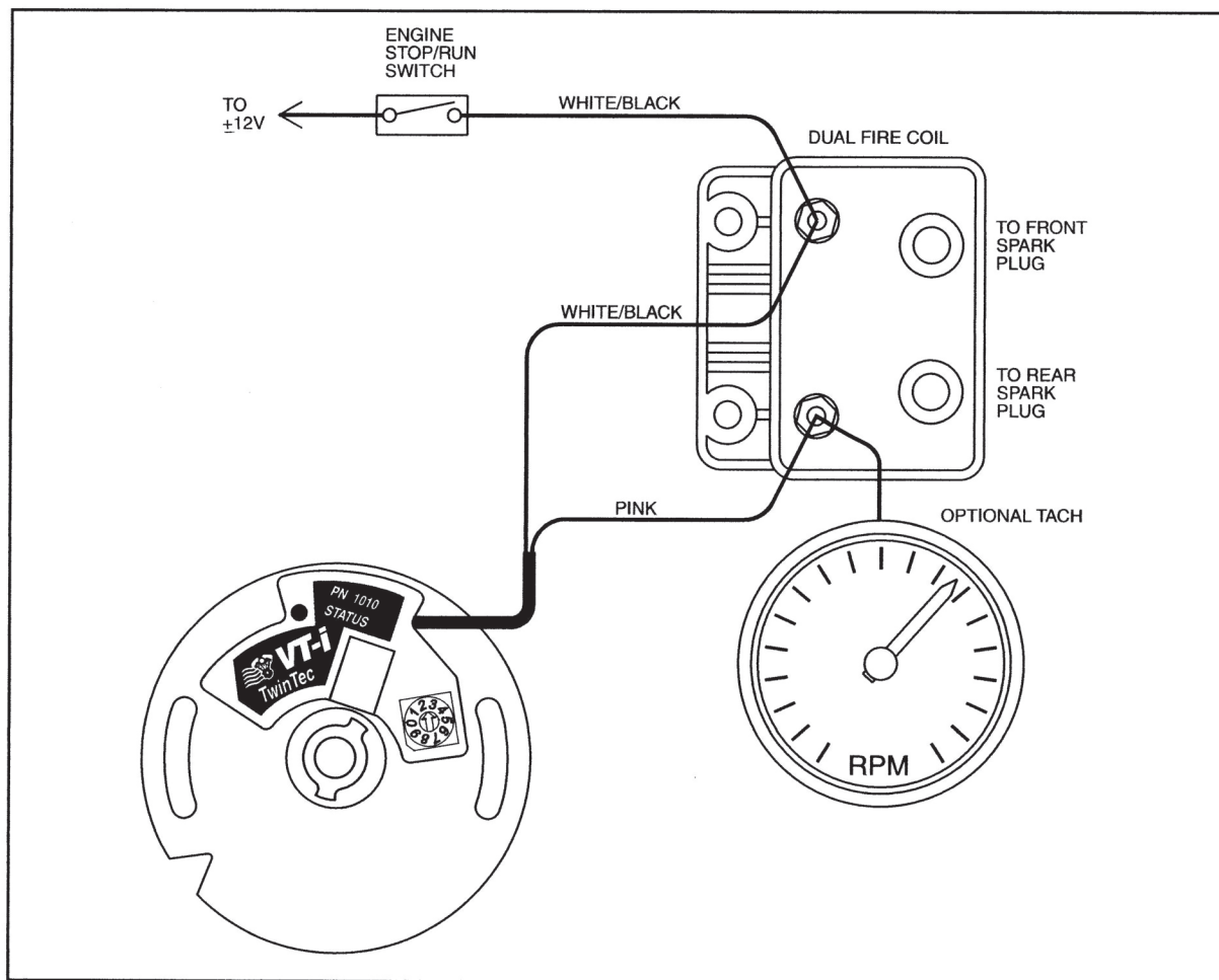
Figure 1 – VT-i Hookup
