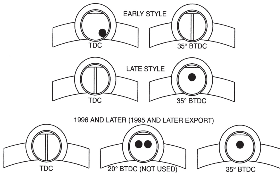
Figure 2 - Front Cylinder Timing Marks
