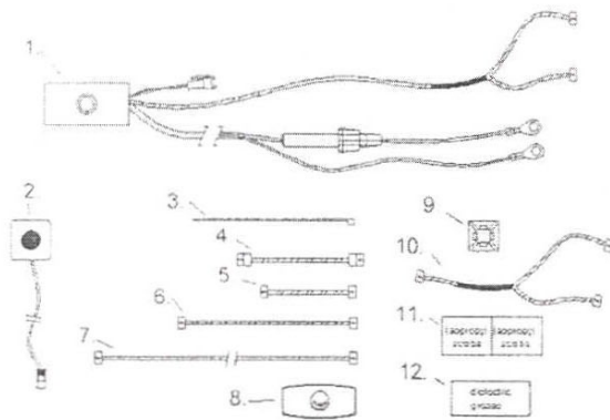
Item description (Qty) - 4 lights Bill of material
