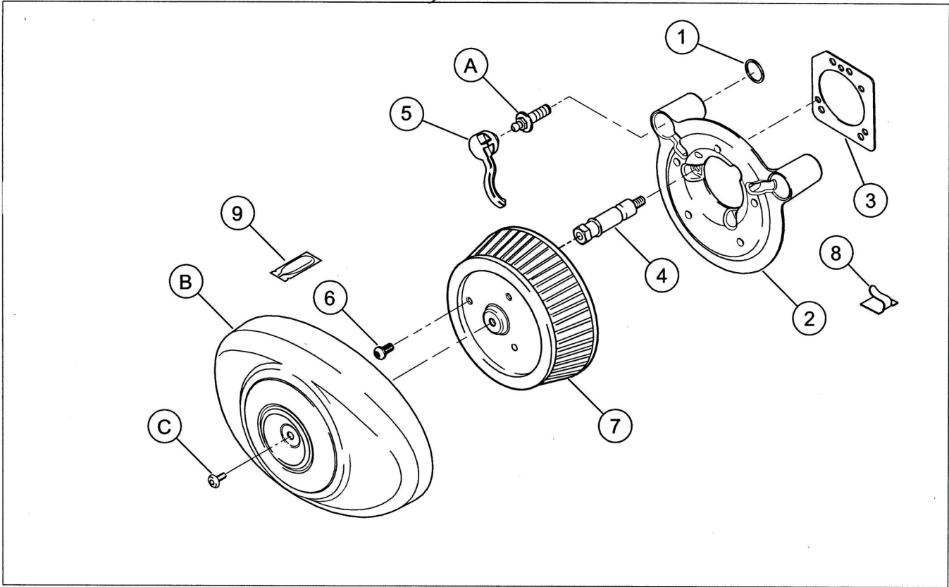
Figure 1. Service Parts: Screamin' Eagle Stage 1 Kit
