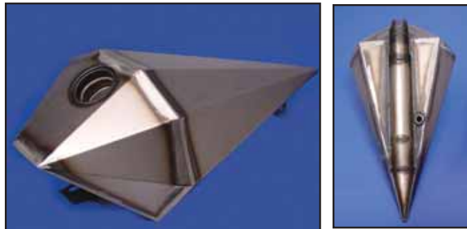
Wyatt's Pirate Tank features mini design allows for full engine view. Measures 22" long with a 19 1/2" tunnel length. 2.2 gallon capacity with front and rear tab mount.
