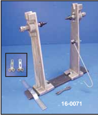
Wheel Truing Fixture of cast alloy construction. Adjustable width for all wheels, with or without axle in place. Order 16-0071 roller stanchions for use with flywheels and
