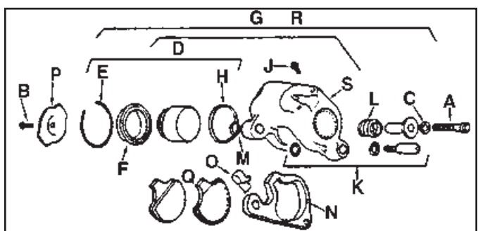
1984-99 Front Calipers and Components.
