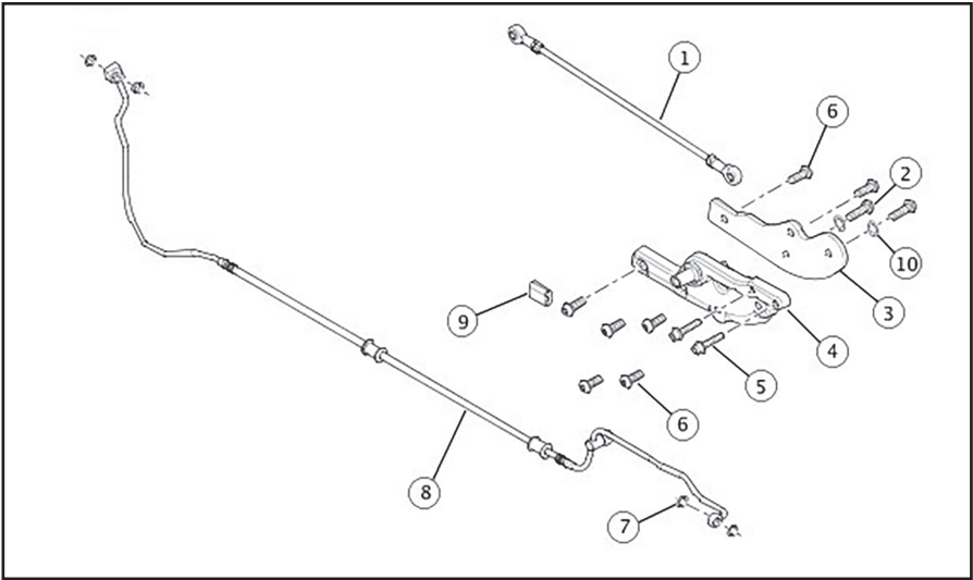
Figure 4. Service Parts: Extended Reach Controls Kit
