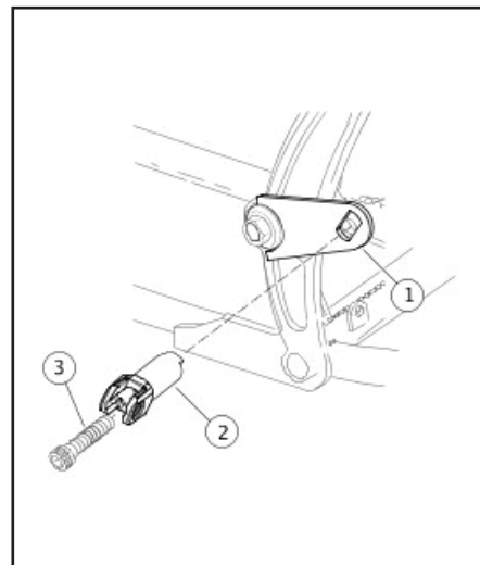
Figure 2. Install Brackets and Footpeg Mounts
