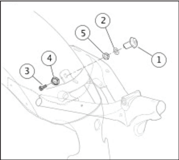
1 Seat post 2 Washer 3 Screw 4 Tee spacer 5 Grommet Figure 1. Seat Post and Mounting Hardware
