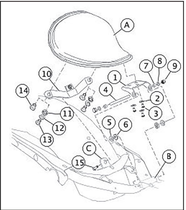
1 Seat post 2 Washer 3 Screw 4 Tee spacer 5 Grommet Figure 1. Seat Post and Mounting Hardware
