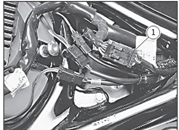
Figure 3. Rear Lighting Harness Connector - Sportster Models
