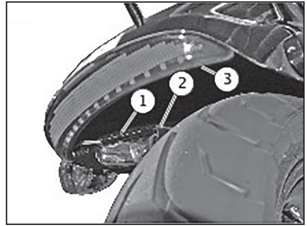
1 Fender edge light wiring harness
