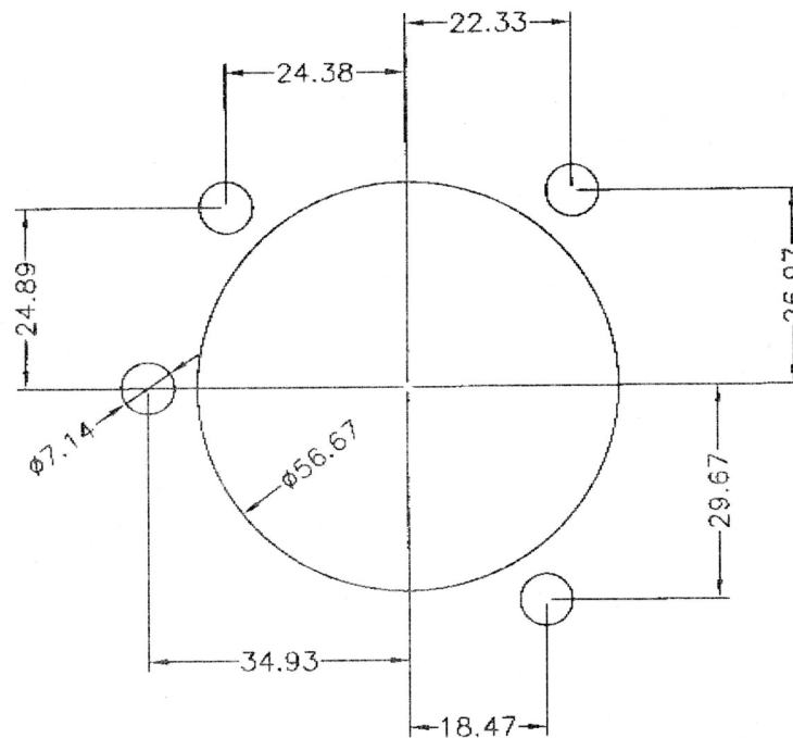
VT No. 34-0746 for VT No. 34-0481 CV
