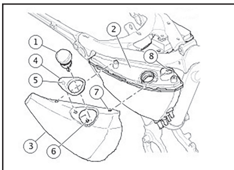
Figure 1. Right Hand Side Cover Installation
