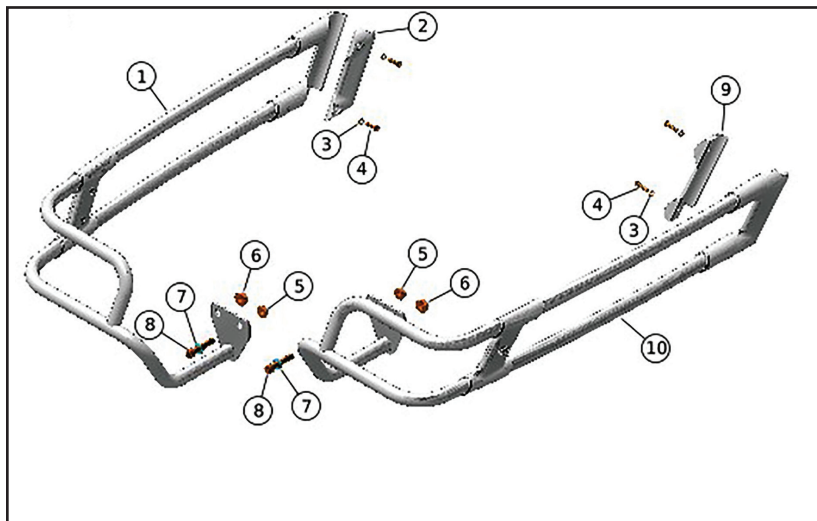
Figure 3. Service Parts: Saddlebag Guard Rail Kit
