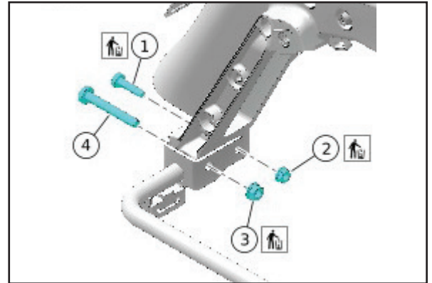
Figure 1. Hardware Removal
