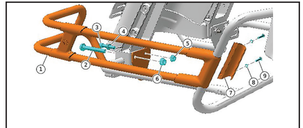
Figure 2. Saddlebag Guard Rail
