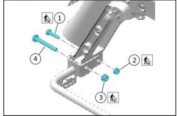
Figure 1. Hardware Removal
