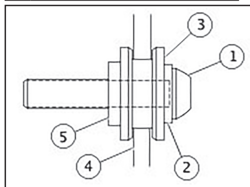
Figure 3. Side Plate and Front Docking Point Fully Engaged
