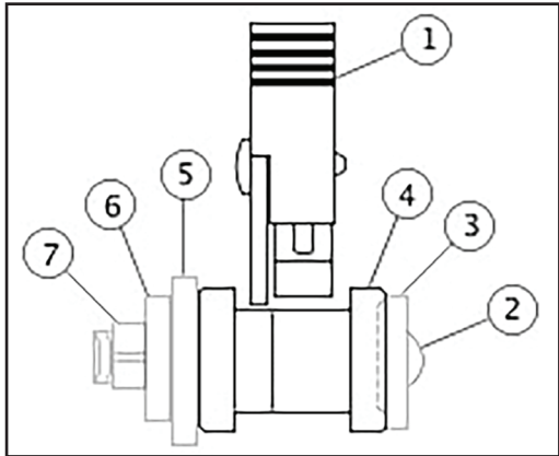
Figure 6. Rear Docking Point Latch Alignment
