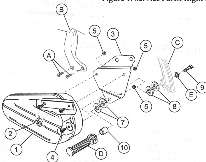
Figure 1. Service Parts: Right Side Toolbox Kit
